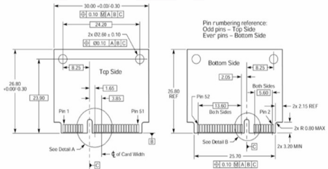
Figure 2-4: Half-Mini Card Top and Bottom
