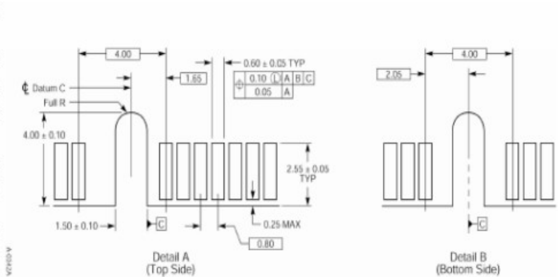
Figure 2-5: Card Top and Bottom Details A and B
